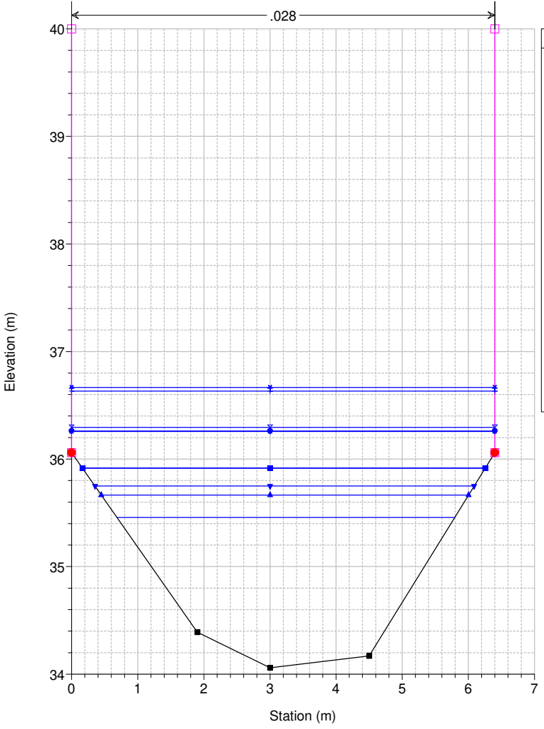
Studio Scandicci Torrenti Greve-Vingone River = Fosso Dogaione Reach = Dogaione RS = 45 DG0010_C
