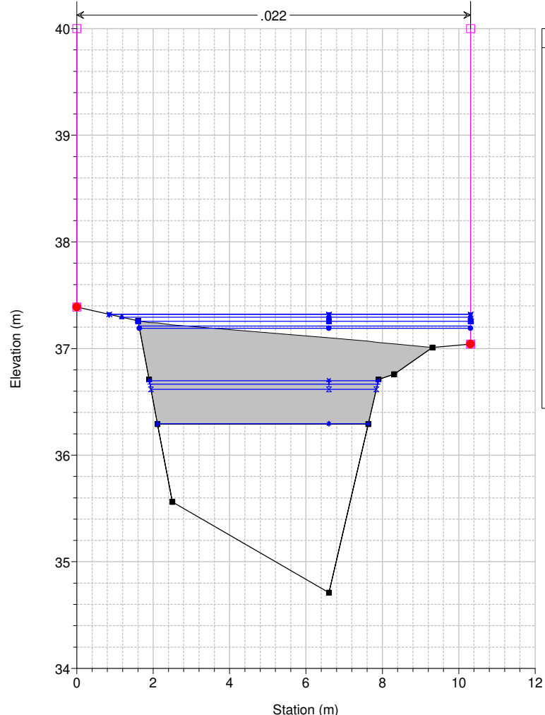
Studio Scandicci Torrenti Greve-Vingone River = Fosso Rigone Reach = Rigone 03 RS = 57 RI0005_C
