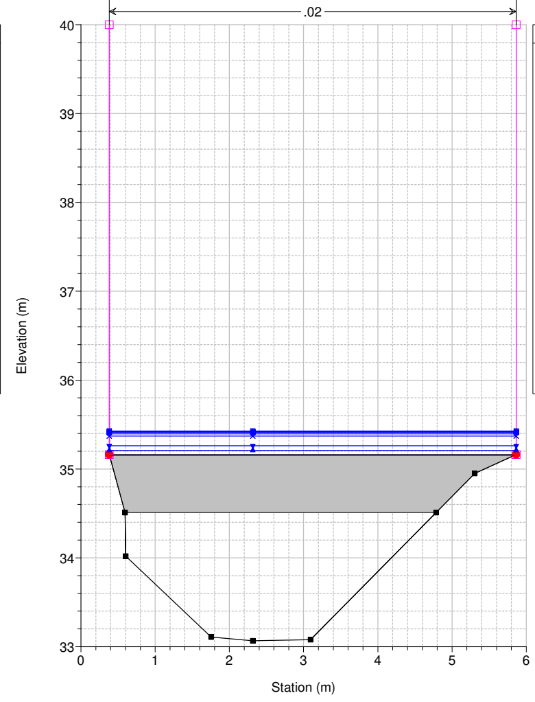
Studio Scandicci Torrenti Greve-Vingone River = Fosso Dogaia Reach = Dogaia_02 RS = 9.5 BR
