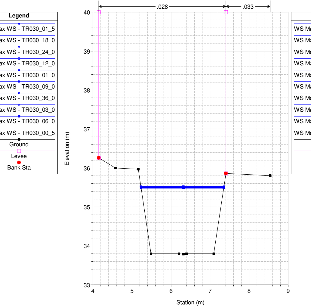
Studio Scandicci Torrenti Greve-Vingone River = Fosso Dogaia Reach = Dogaia_02 RS = 37 DO1016_C
