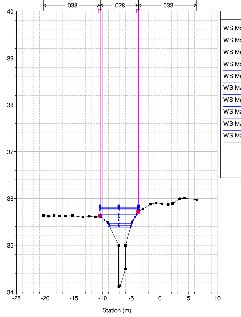
Studio Scandicci Torrenti Greve-Vingone River = Fosso Dogaione Reach = Dogaione RS = 49 DG0009_C
