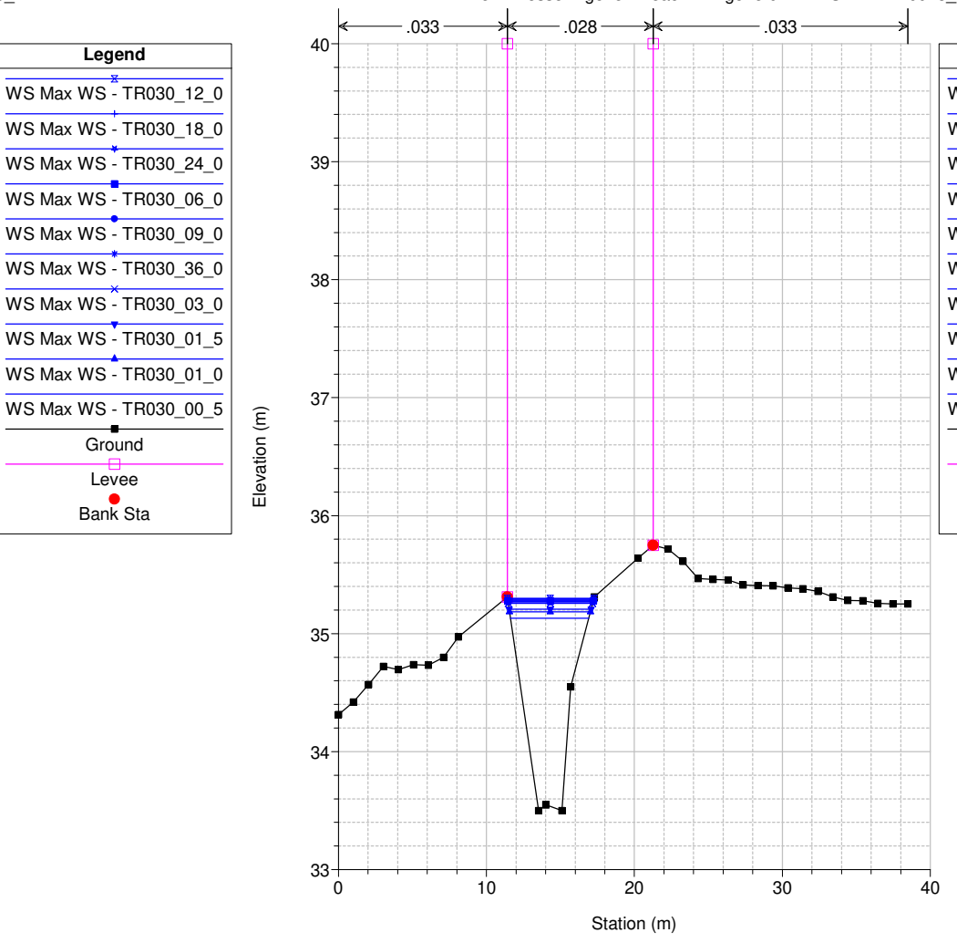
Studio Scandicci Torrenti Greve-Vingone River = Fosso Rigone Reach = Rigone 02 RS = 24 RI0018_B
