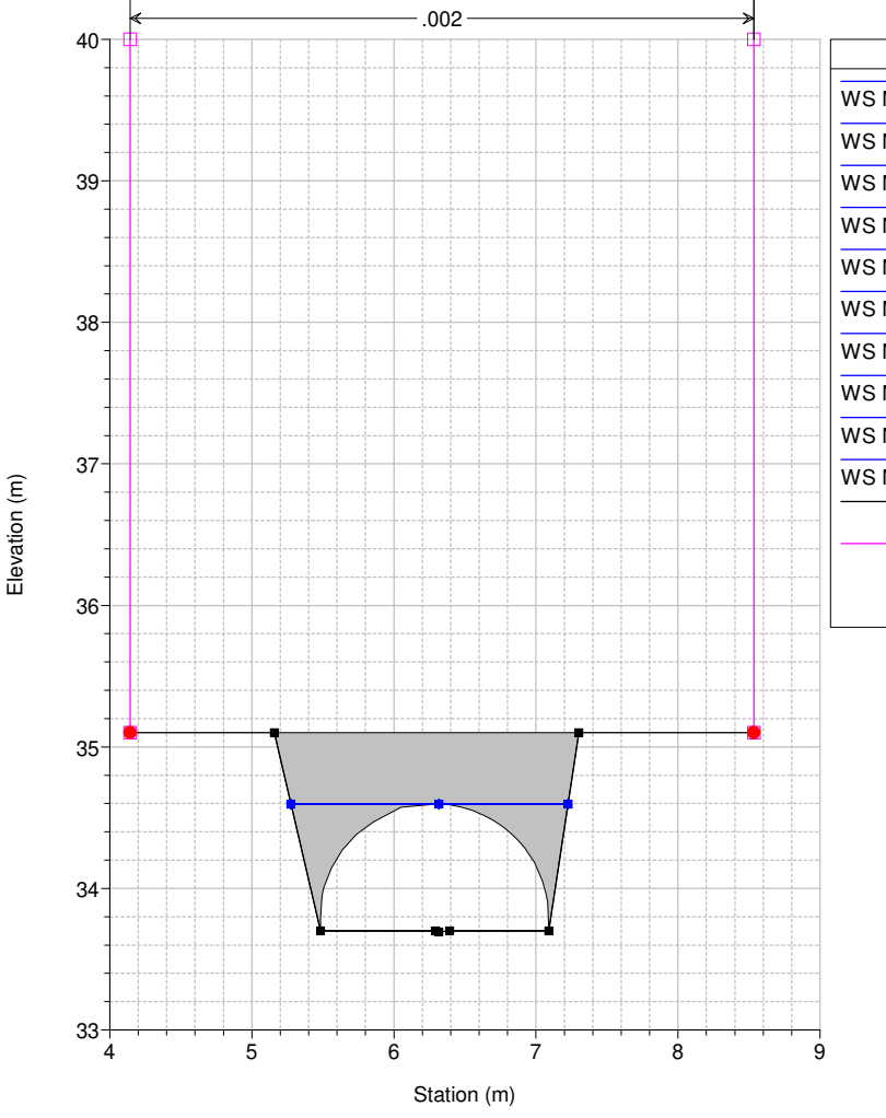
Studio Scandicci Torrenti Greve-Vingone River = Fosso Dogaia Reach = Dogaia_02 RS = 37.5 BR
