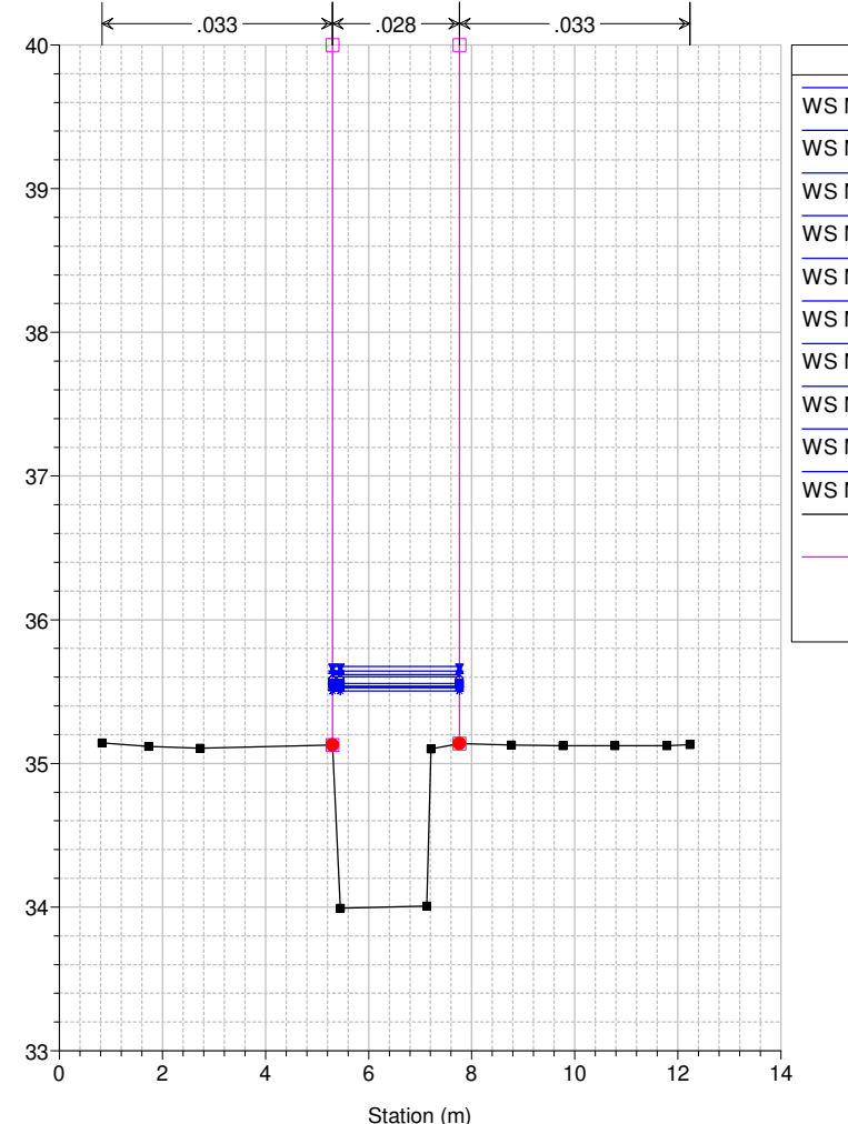
Studio Scandicci Torrenti Greve-Vingone River = Fosso Dogaia Reach = Dogaia_02 RS = 41.5 BR
