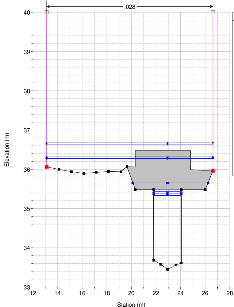
Studio Scandicci Torrenti Greve-Vingone River = Fosso Dogaia Reach = Dogaia_02 RS = 11 DO0024_A
