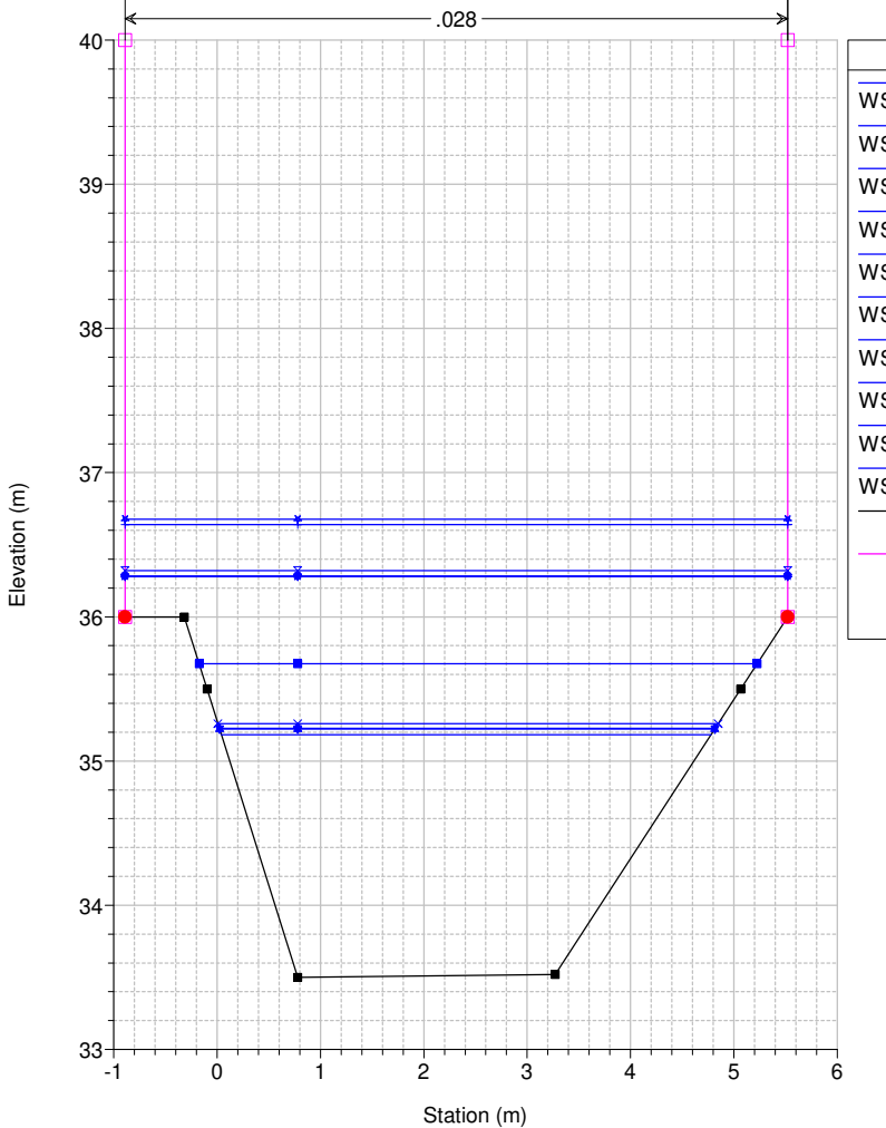
Studio Scandicci Torrenti Greve-Vingone River = Fosso Rigone Reach = Rigone 02 RS = 15 RI0021_B
