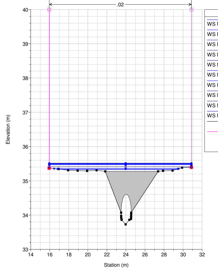
Studio Scandicci Torrenti Greve-Vingone River = Fosso Dogaia Reach = Dogaia_02 RS = 33.5 BR
