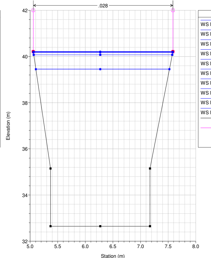
Studio Scandicci Torrenti Greve-Vingone River = Fosso Dogaione Reach = Dogaione RS = 2 DG0018_C
