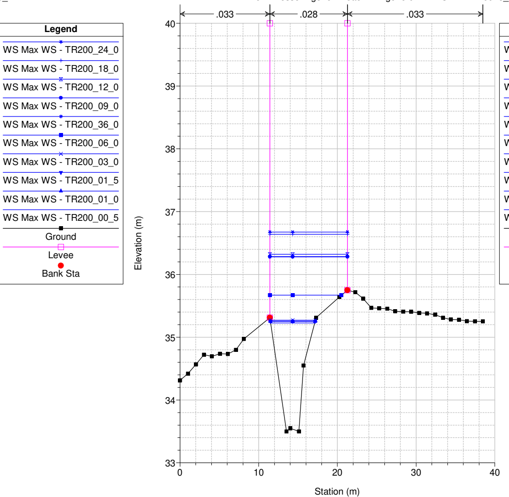
Studio Scandicci Torrenti Greve-Vingone River = Fosso Rigone Reach = Rigone 02 RS = 24 RI0018_B
