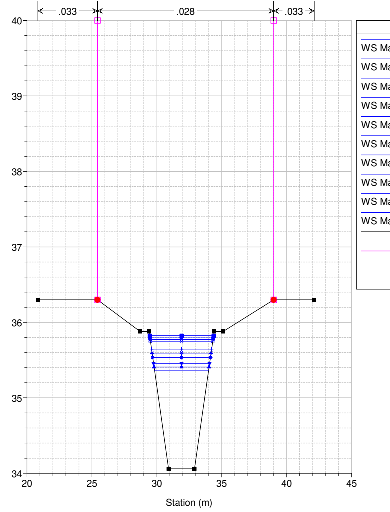
Studio Scandicci Torrenti Greve-Vingone River = Fosso Dogaione Reach = Dogaione RS = 29 DG1014_C
