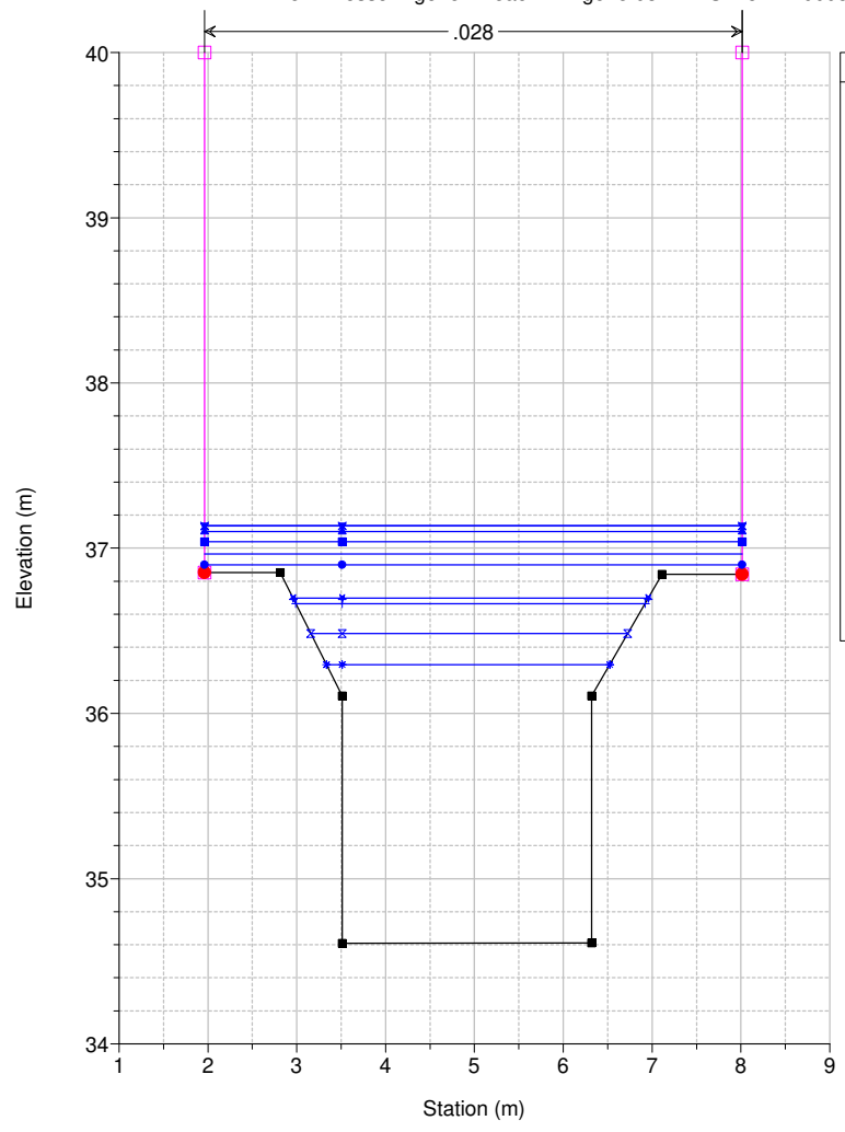
Studio Scandicci Torrenti Greve-Vingone River = Fosso Rigone Reach = Rigone 03 RS = 57 RI0005_C
