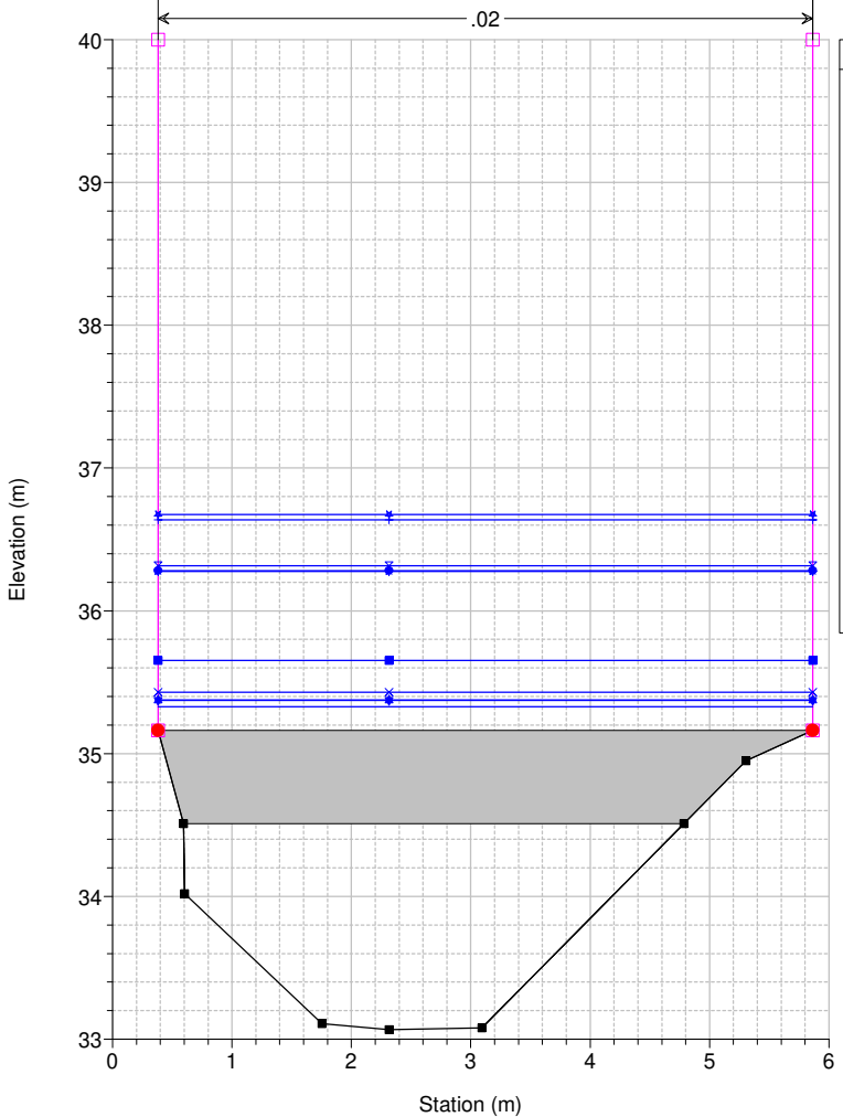
Studio Scandicci Torrenti Greve-Vingone River = Fosso Dogaia Reach = Dogaia_02 RS = 9.5 BR
