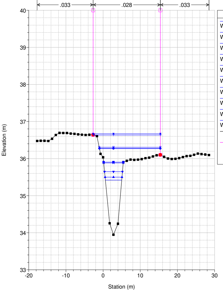
Studio Scandicci Torrenti Greve-Vingone River = Fosso Dogaione Reach = Dogaione RS = 23 DG0013_A
