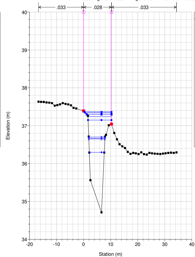
Studio Scandicci Torrenti Greve-Vingone River = Fosso Rigone Reach = Rigone 03 RS = 58 RI0005_B
