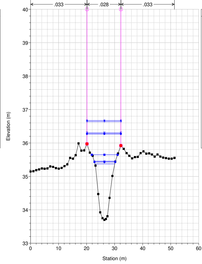
Studio Scandicci Torrenti Greve-Vingone River = Fosso Dogaia Reach = Dogaia_02 RS = 23 DO1021_A
