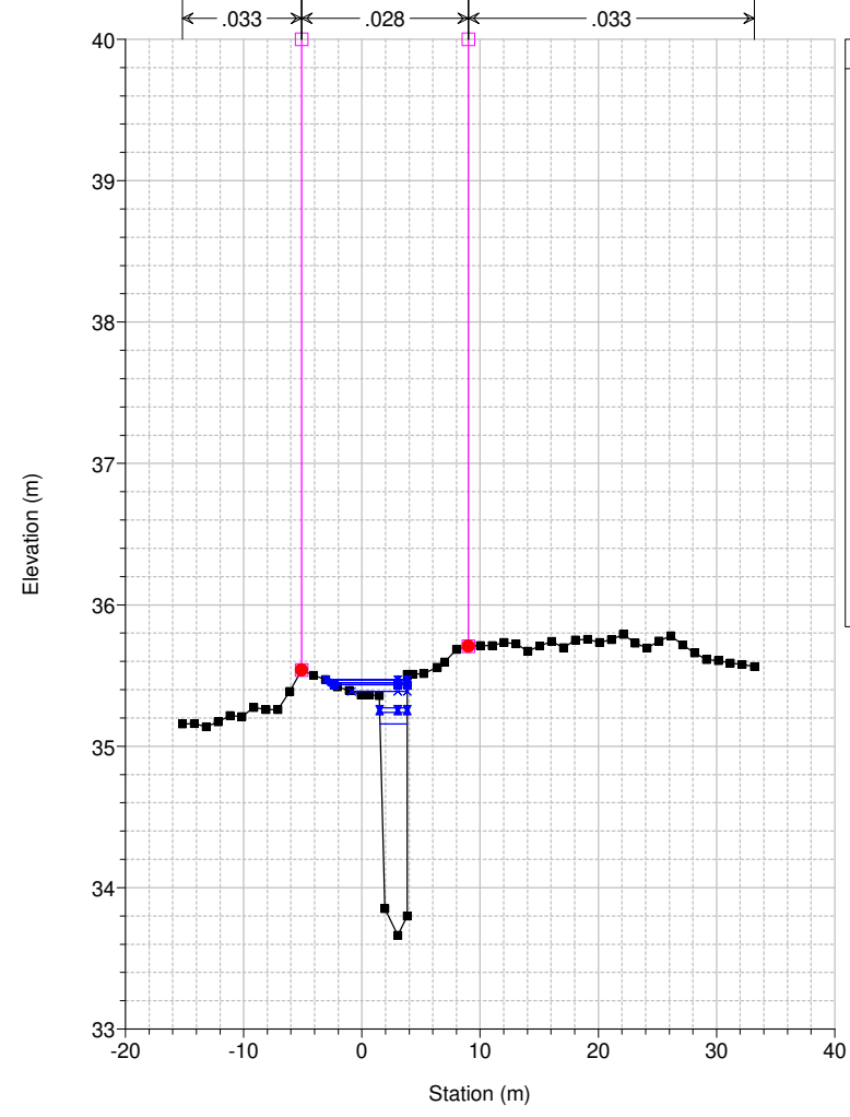
Studio Scandicci Torrenti Greve-Vingone River = Fosso Dogaia Reach = Dogaia_02 RS = 25 DO1020_D
