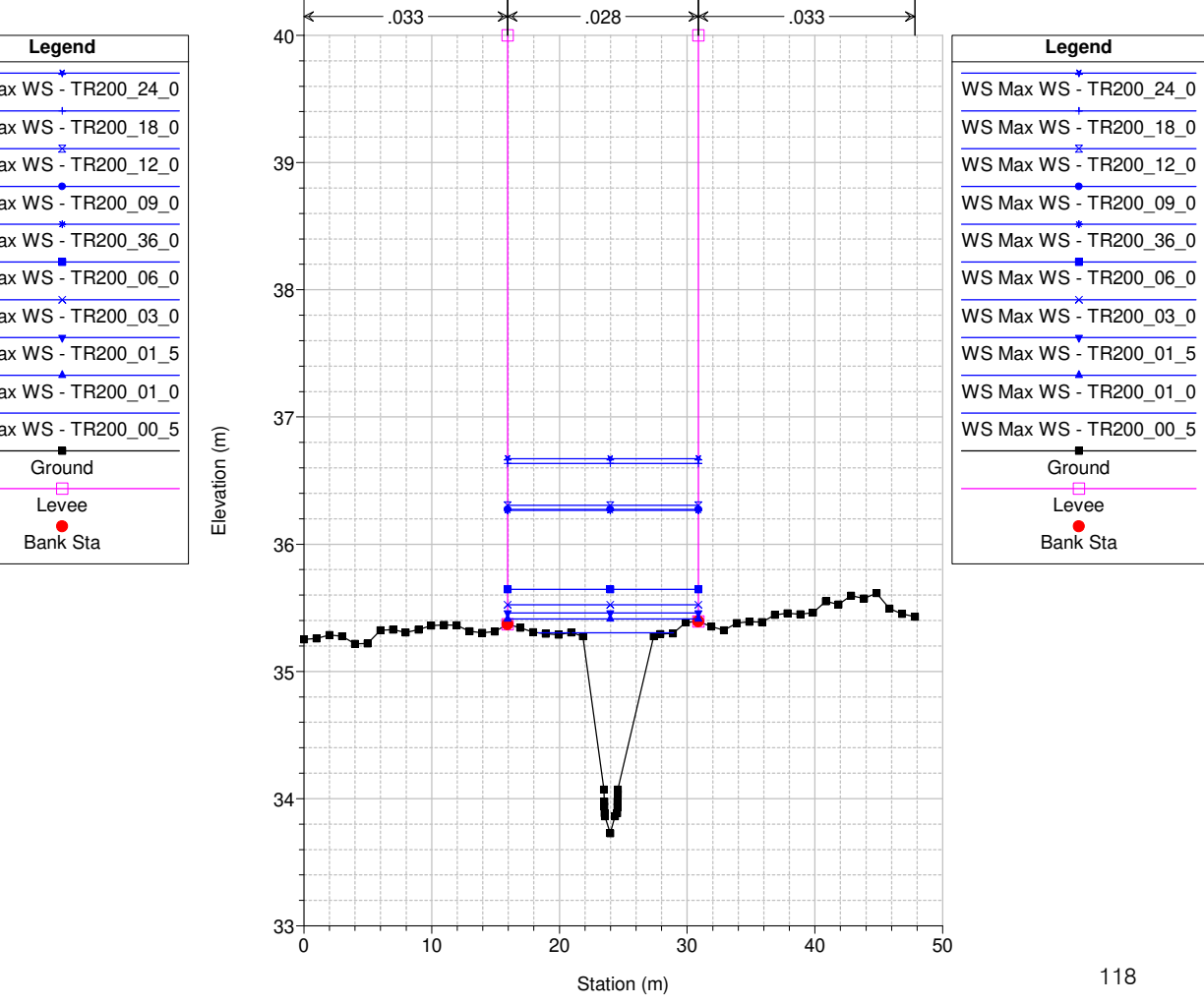
Studio Scandicci Torrenti Greve-Vingone River = Fosso Dogaia Reach = Dogaia_02 RS = 33 DO1017_C
