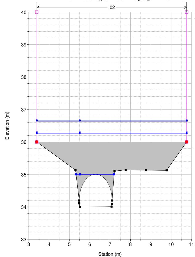
Studio Scandicci Torrenti Greve-Vingone River = Fosso Dogaia Reach = Dogaia_02 RS = 41.5 BR
