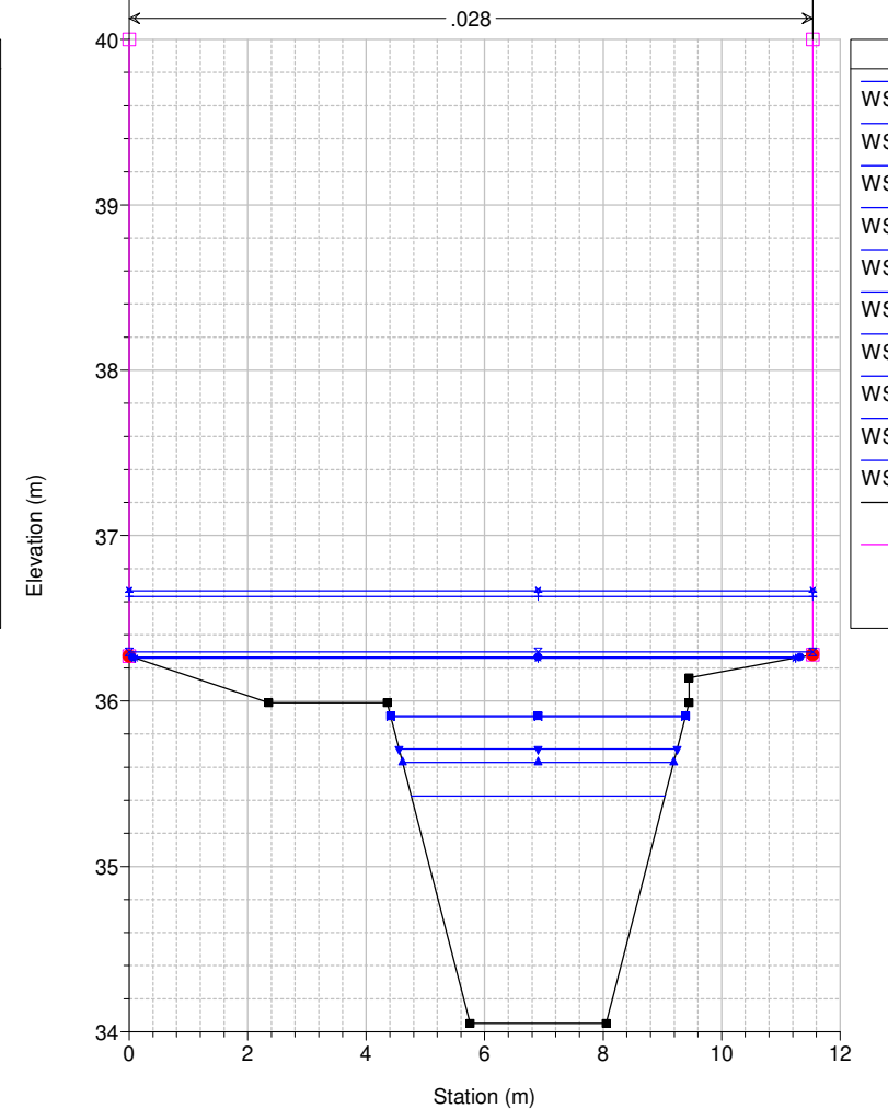
Studio Scandicci Torrenti Greve-Vingone River = Fosso Dogaione Reach = Dogaione RS = 40 DG1011_D
