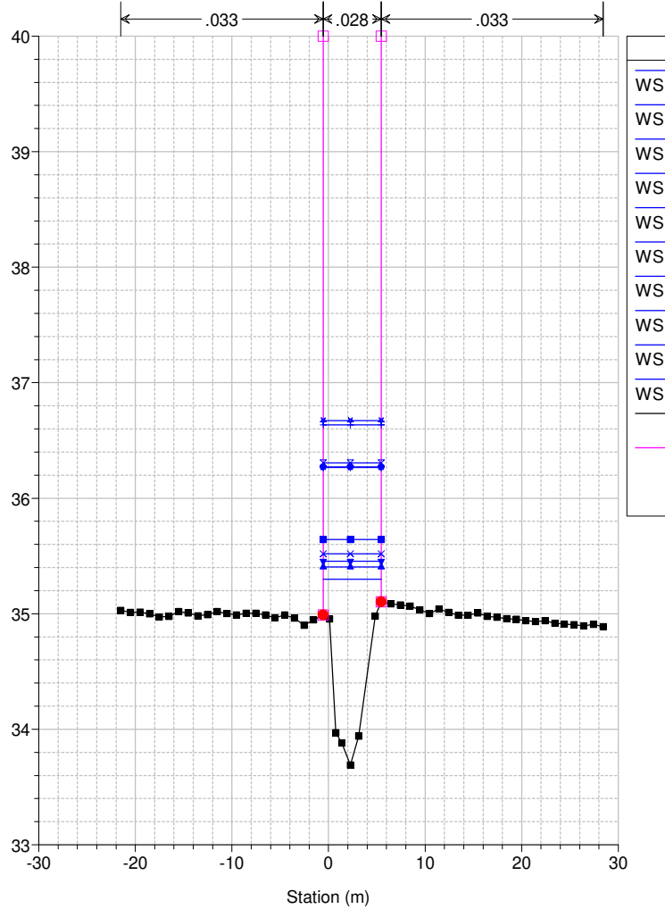
Studio Scandicci Torrenti Greve-Vingone River = Fosso Dogaia Reach = Dogaia_02 RS = 28 DO1020_A
