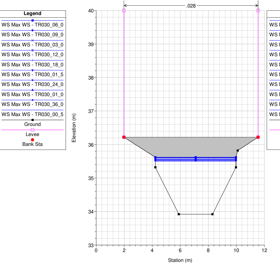
Studio Scandicci Torrenti Greve-Vingone River = Fosso Dogaione Reach = Dogaione RS = 57 DG1006_D
