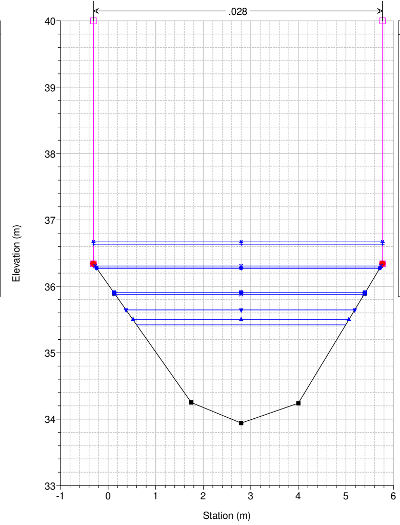
Studio Scandicci Torrenti Greve-Vingone River = Fosso Dogaione Reach = Dogaione RS = 18 DG0014_B
