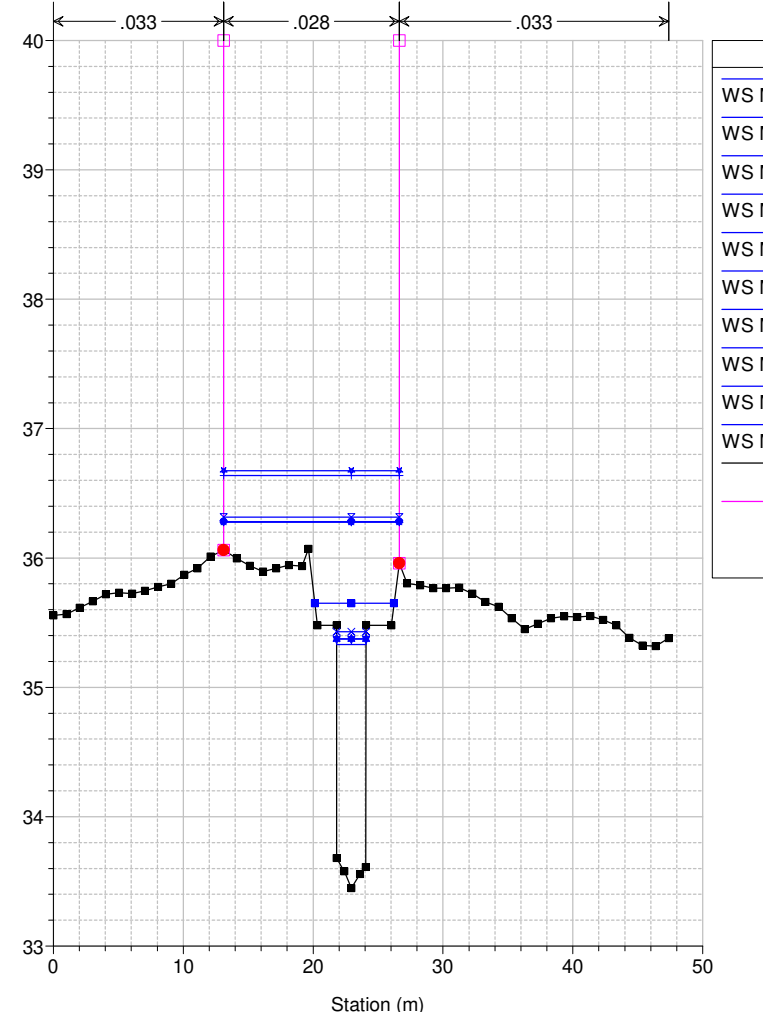
Studio Scandicci Torrenti Greve-Vingone River = Fosso Dogaia Reach = Dogaia_02 RS = 10 DO0024_B
