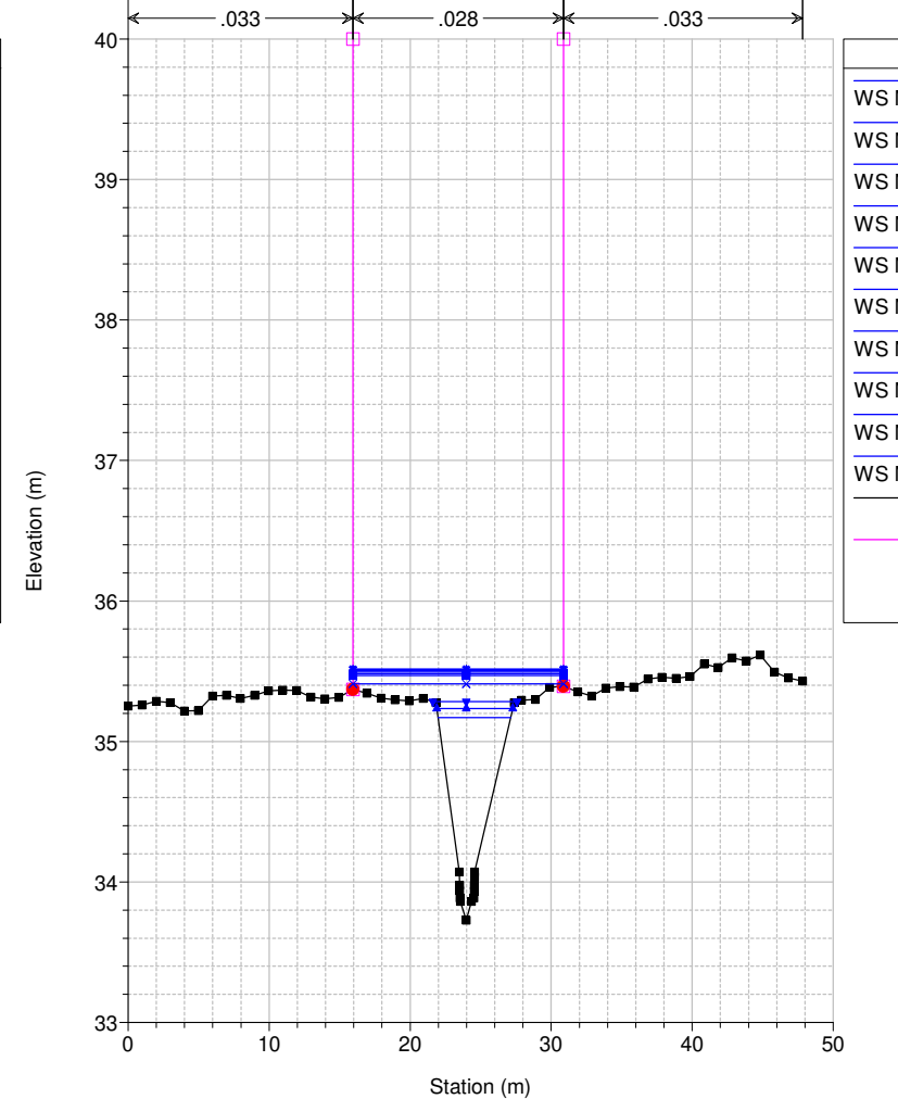
Studio Scandicci Torrenti Greve-Vingone River = Fosso Dogaia Reach = Dogaia_02 RS = 33 DO1017_C
