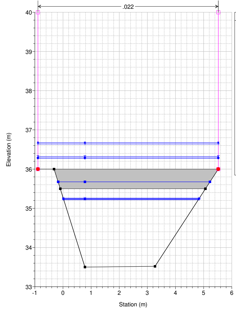
Studio Scandicci Torrenti Greve-Vingone River = Fosso Rigone Reach = Rigone 02 RS = 14 R10021_C
