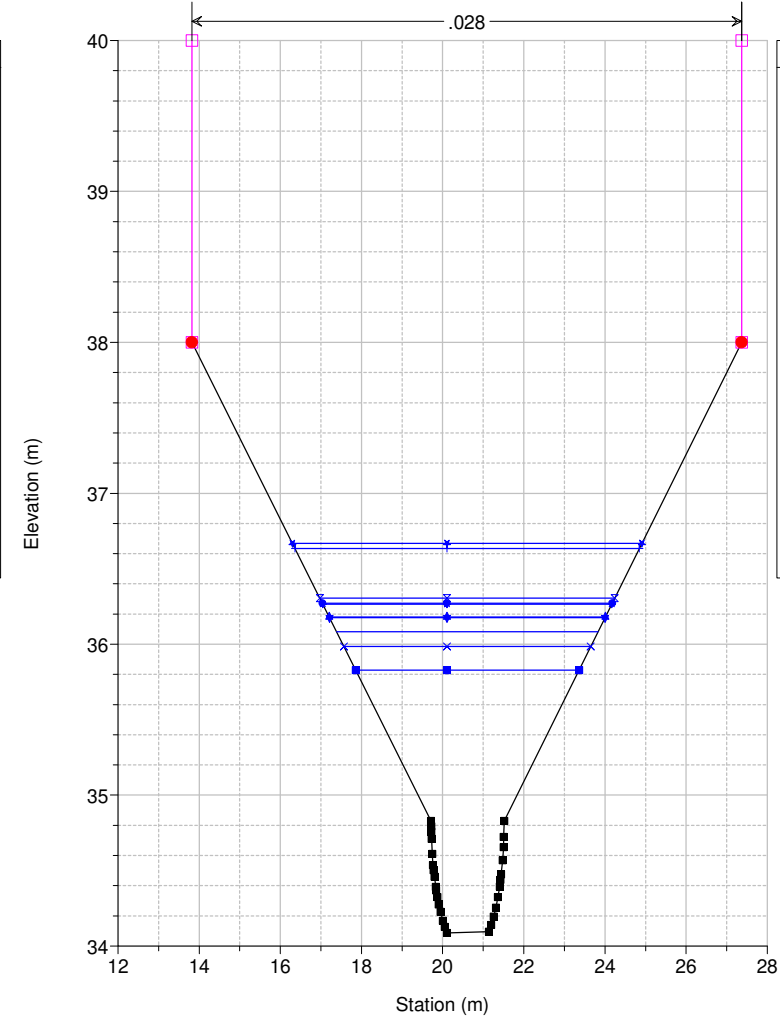
Studio Scandicci Torrenti Greve-Vingone River = Fosso Dogaia Reach = Dogaia_02 RS = 45 DO1014_C
