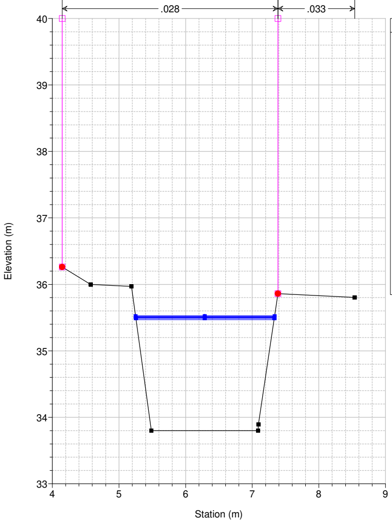
Studio Scandicci Torrenti Greve-Vingone River = Fosso Dogaia Reach = Dogaia_02 RS = 41 DO1015_C
