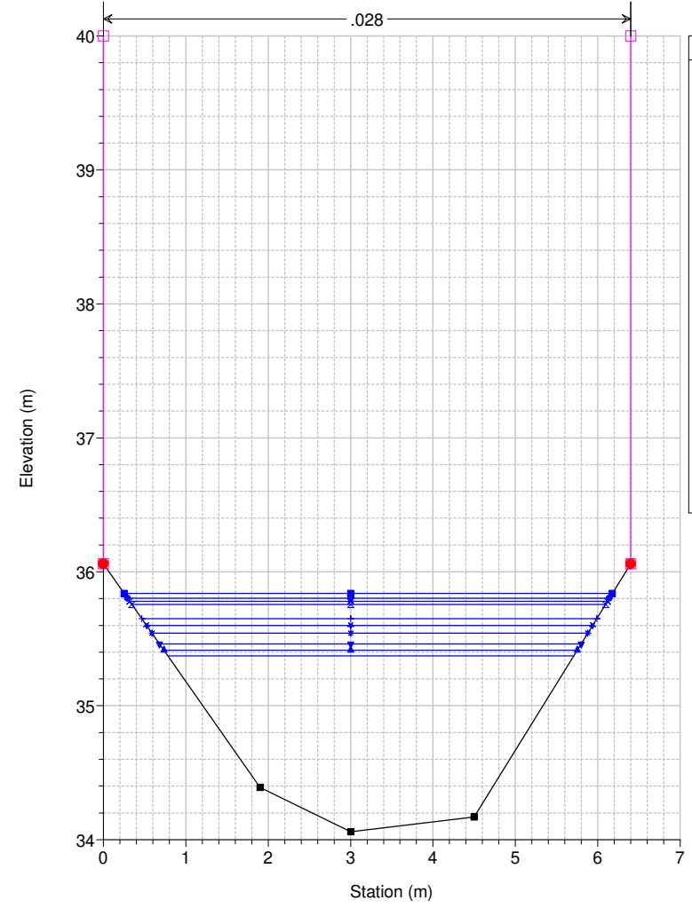
Studio Scandicci Torrenti Greve-Vingone River = Fosso Dogaione Reach = Dogaione RS = 45 DG0010_C
