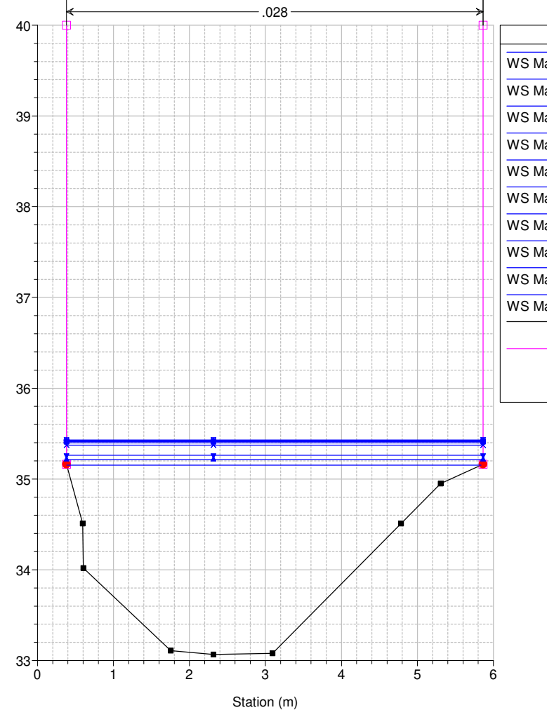
Studio Scandicci Torrenti Greve-Vingone River = Fosso Dogaia Reach = Dogaia_02 RS = 10 DO0024_B
