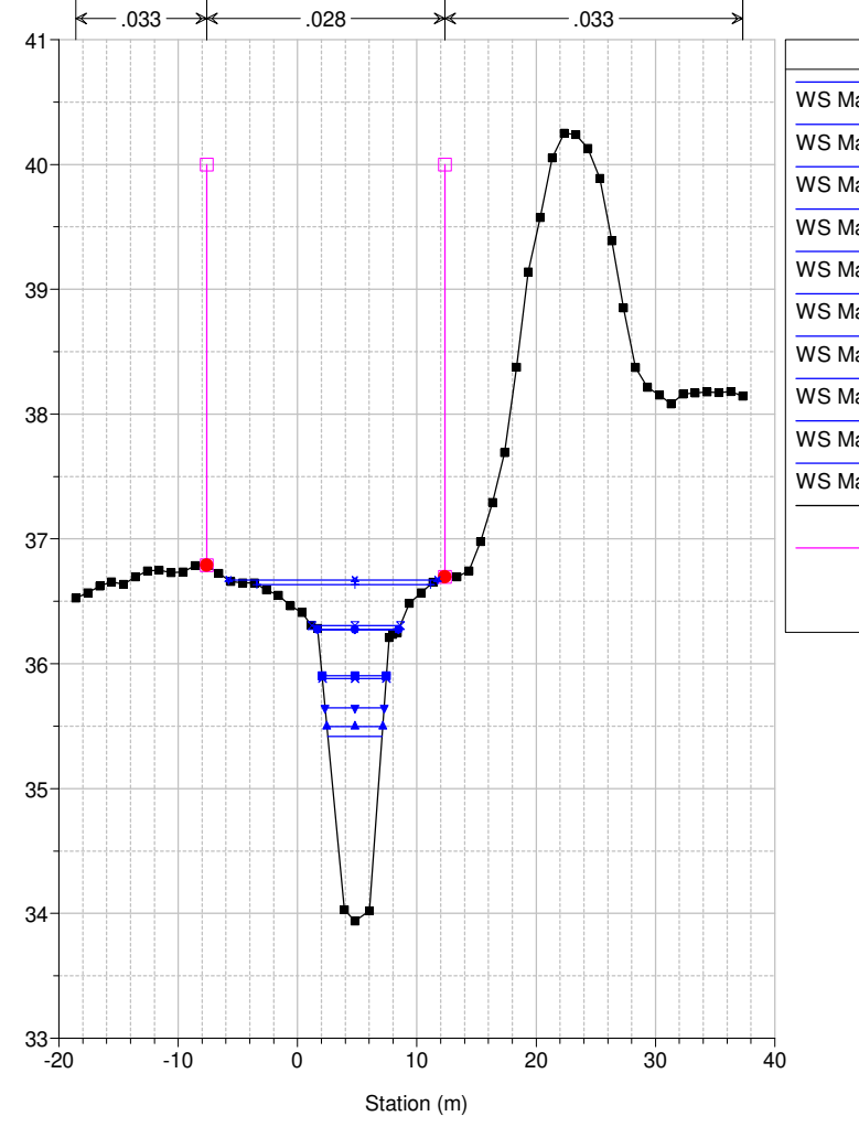
Studio Scandicci Torrenti Greve-Vingone River = Fosso Dogaione Reach = Dogaione RS = 19 DG0014_A
