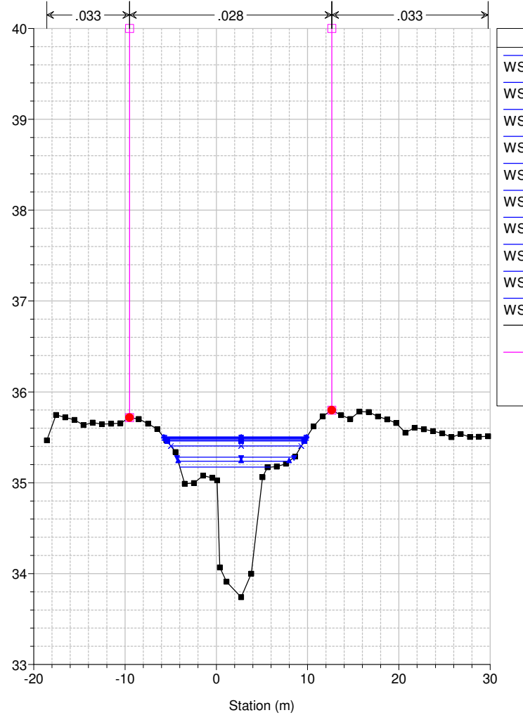
Studio Scandicci Torrenti Greve-Vingone River = Fosso Dogaia Reach = Dogaia_02 RS = 27 DO1020_B
