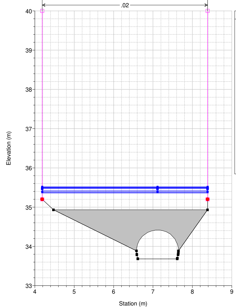
Studio Scandicci Torrenti Greve-Vingone River = Fosso Dogaia Reach = Dogaia_02 RS = 33.5 BR
